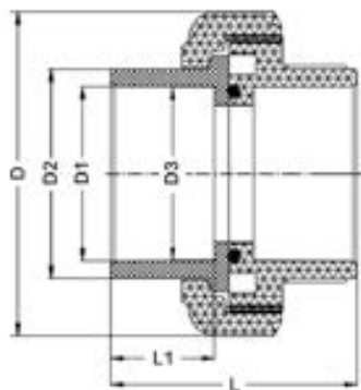
Муфта ХПВХ IPS (Model A) d90 PN16
