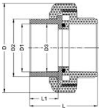
Муфта ХПВХ IPS (Model A) d50 PN16
