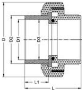
Муфта ХПВХ IPS (Model A) d75 PN16
