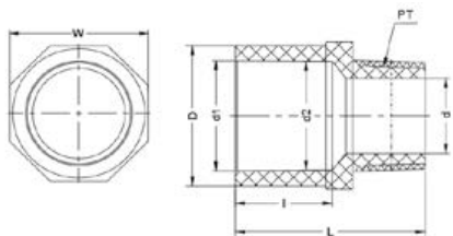
Муфта ХПВХ IPS 20x1/2" PN16
