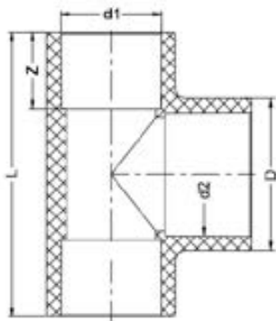
Тройник 90° ХПВХ IPS (Model B) d500 PN10
